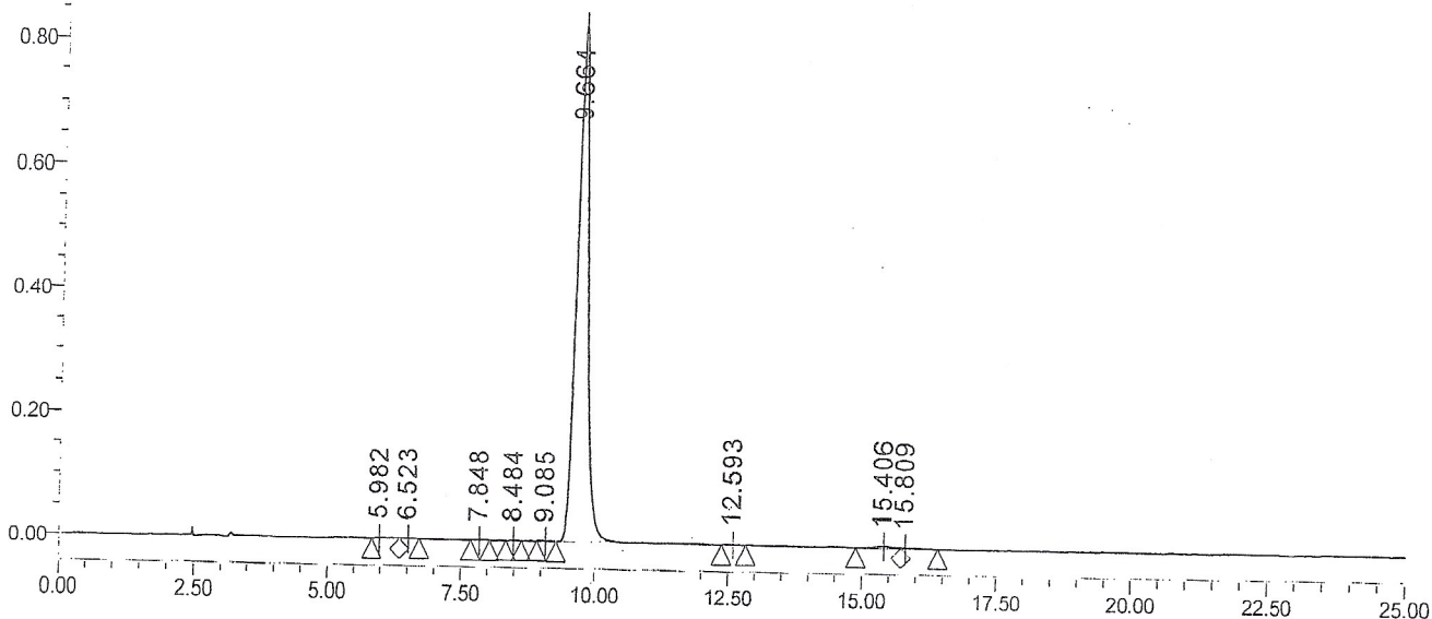
Auto-Scaled Chromatogram
